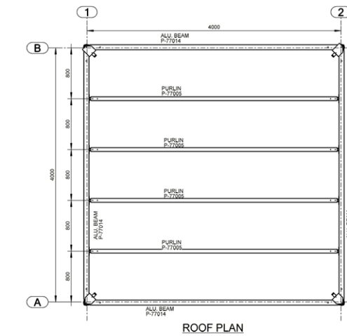
ROOF PLAN
