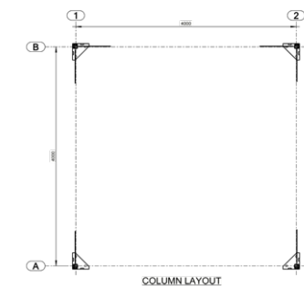
COLUMN LAYOUT
